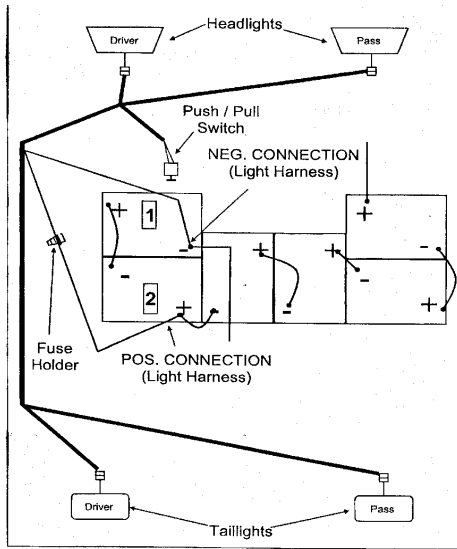
Club Car Basic 36-Volt Wiring Diagram
