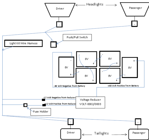
Club Car Basic 48-Volt Wiring Diagram
